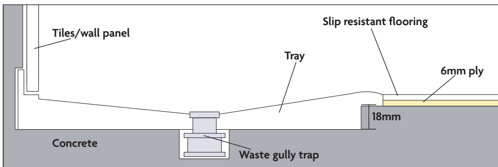
Level access concrete
