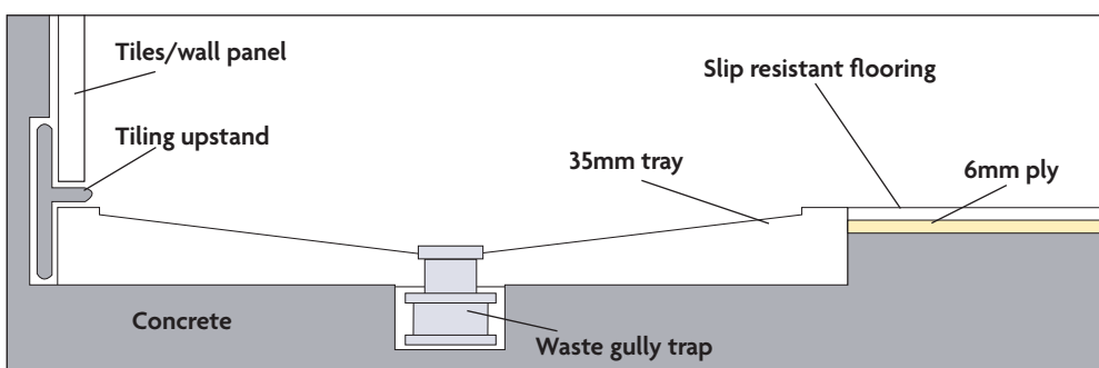
Easy access recessed into concrete
