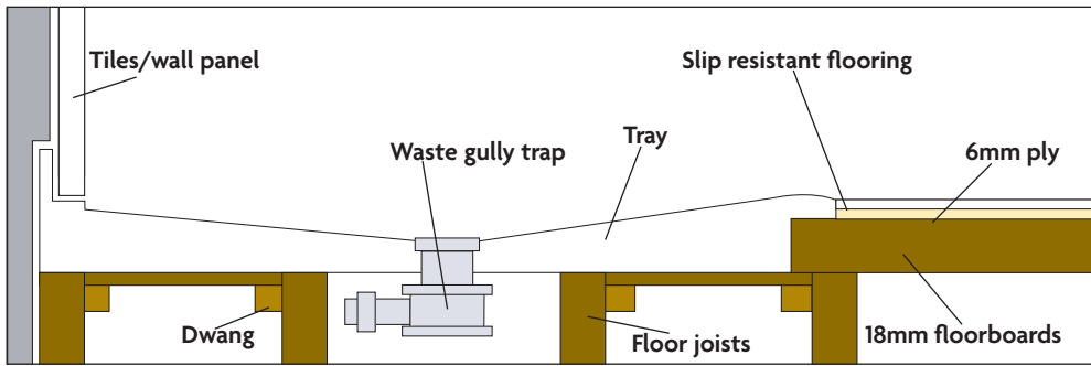
Level access timber
