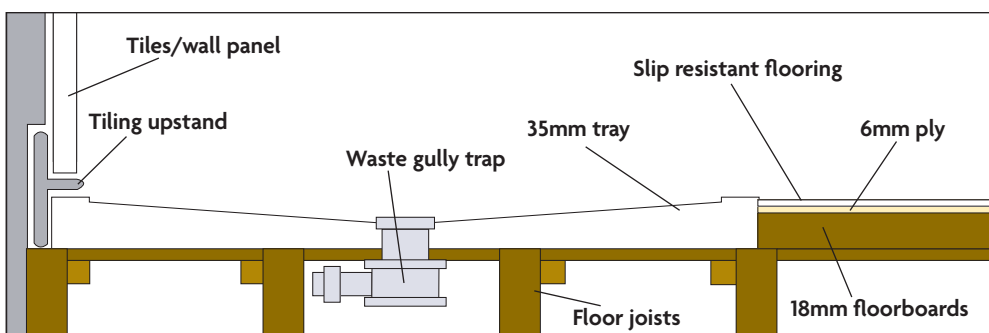
Easy access recessed into timber
